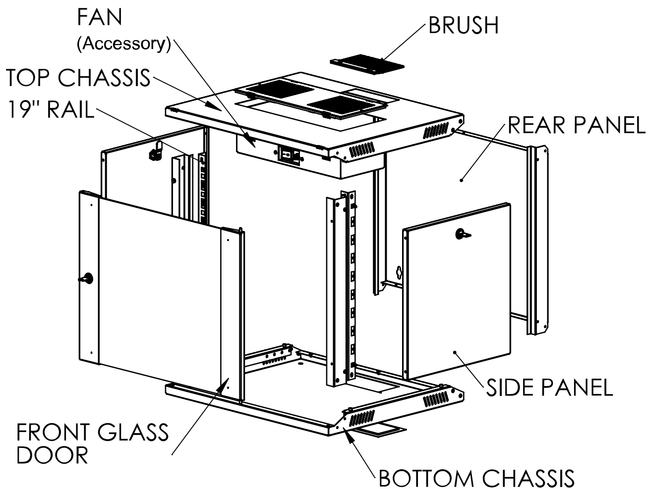
Exploded view
