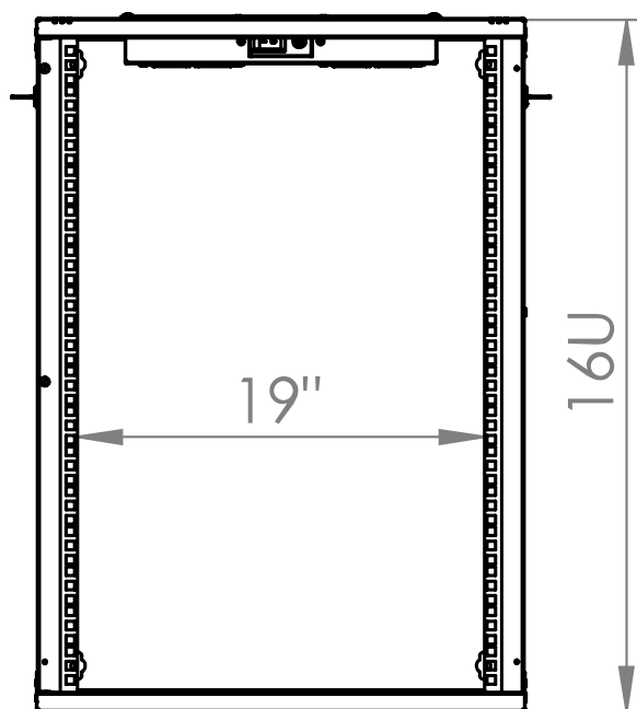
Front inside view
